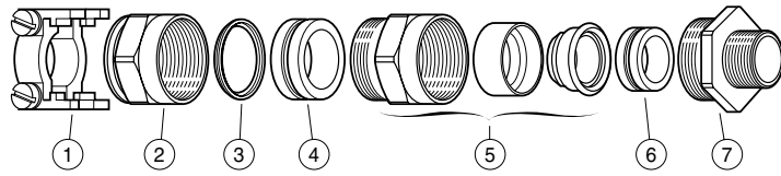
1/2 - 3/4 NPT, for armoured cable
